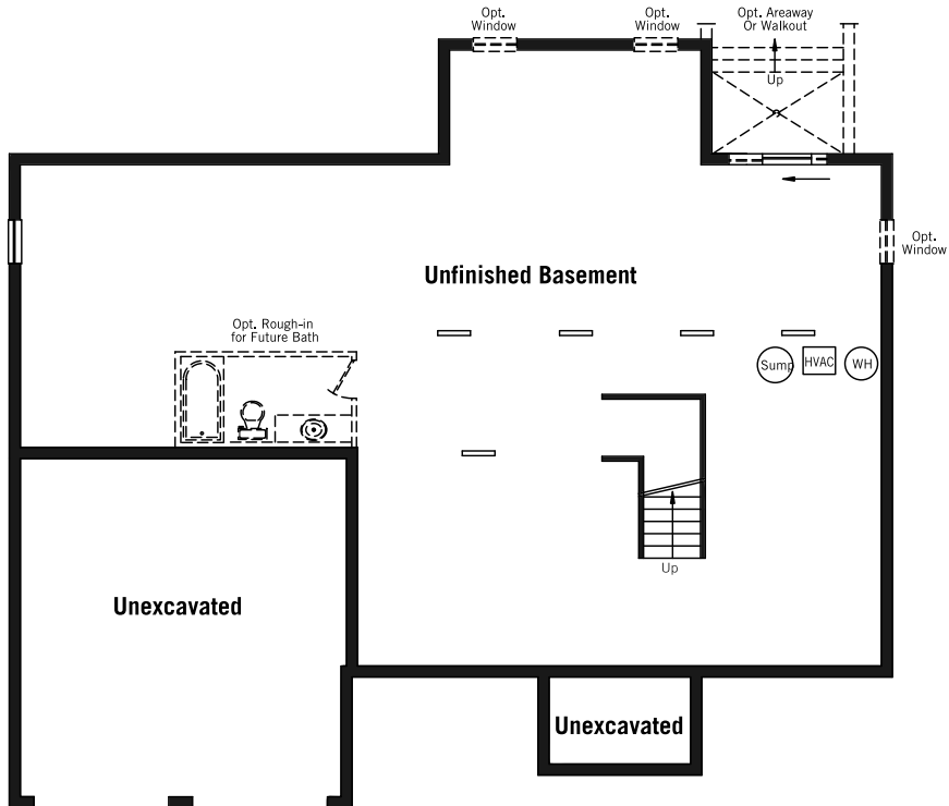
Unfinished Basement Plan
