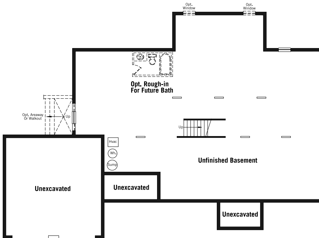
Unfinished Basement Plan
