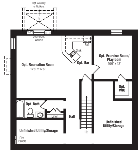
Optional Finished Lower Level
