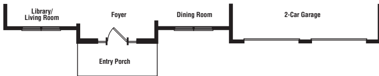
Partial First Floor Plan w/Elev. 2
