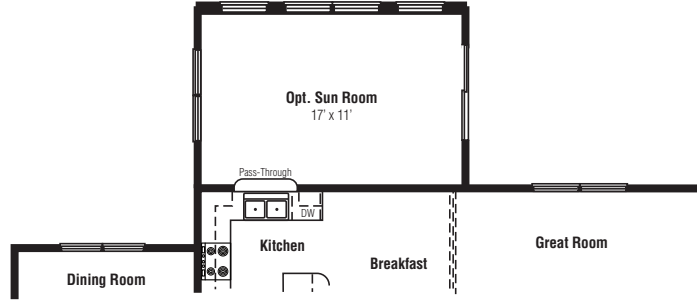
Partial First Floor Plan w/Opt. Sun Room
