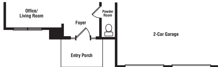
Partial First Floor Plan w/Elev. 2
